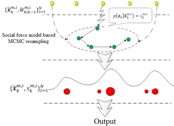
Fig. 2. The basic operation of the proposed social force model-aided MCMC based particle filter.
