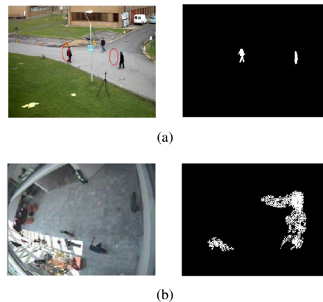
Fig. 7. Selected examples of failure cases of the proposed tracking system. In (a) the tracking results are influenced by the failure of detection from background subtraction; and (b) the brightness of the environment causes the failure of the background subtraction.
