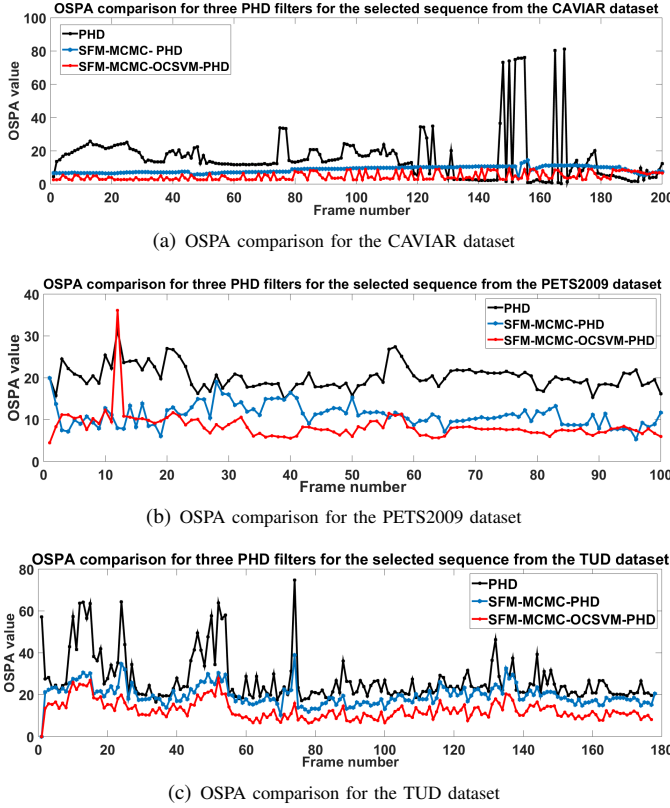
Fig. 6. Performance evaluation with OSPA measure for our proposed social force model aided MCMC particle PHD filter and the traditional particle PHD filter for multiple human tracking. The performance is examined with the ‘EnterExitCrossingPaths1cor’ sequence from the CAVIAR dataset, the ‘PETS09_View001_S2_L1’ sequence from the PETS2009 dataset and the ‘TUD_Stadtmitte’ sequence from the TUD dataset. The black line in the figure denotes the OSPA value from the traditional PHD particle PHD filter; the blue line shows the result by adding a social force model aided MCMC resampling step in the prediction stage of the particle PHD filter; and the red line denotes the OSPA value from our proposed SFM-MCMC-OCSVM-PHD filter.
