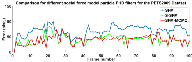
(b) Social force model comparison for the PETS2009 dataset
