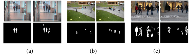
Fig. 3. Selected frames and examples for background subtraction results from the three selected sequences from three different datasets, i.e. (a) is from the 'EnterExitCrossingPaths1cor' sequence from the CAVIAR dataset, (b) is from the 'PETS09_View001_S2_L1' sequence from the PETS2009 dataset and (c) is from 'TUD_Stadtmitte' sequence from the TUD dataset, where we can find the human target boundaries are extracted successfully, but there is still much environmental noise which may cause missed detections and false alarms. In order to mitigate such noise, an OCSVM classifier will be employed based upon the features from both color and oriented gradient histograms of human targets.
