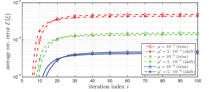
Fig. 4. Ensemble reconstruction error E\{\xi\} vs. SBR2 iterations for the different truncation approaches and varying \mu .
