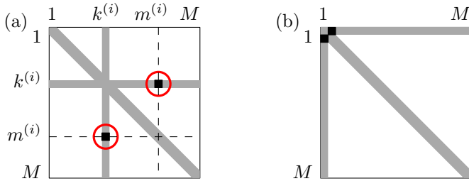
Fig. 1. Sparsity structure of lag zero matrix \mathbf{S}^{(i)'}[0] after i th iteration of (a) the SMD algorithm, indicating the maximum off-diagonal element in position m^{(i)} of the k^{(i)} th row, and (b) after permutation.
