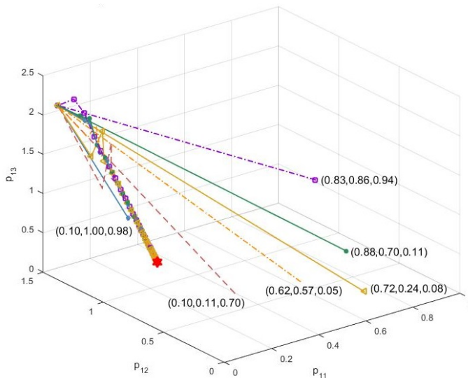
Fig. 5: Convergence of power allocation of player 1 for different starting strategies when K = 4 and M = 3 , second simulation (different linestyles correspond to different initial strategies for player 1).
