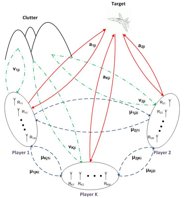
Fig. 1: A distributed MIMO radar network with K clusters and their corresponding channel gains.
