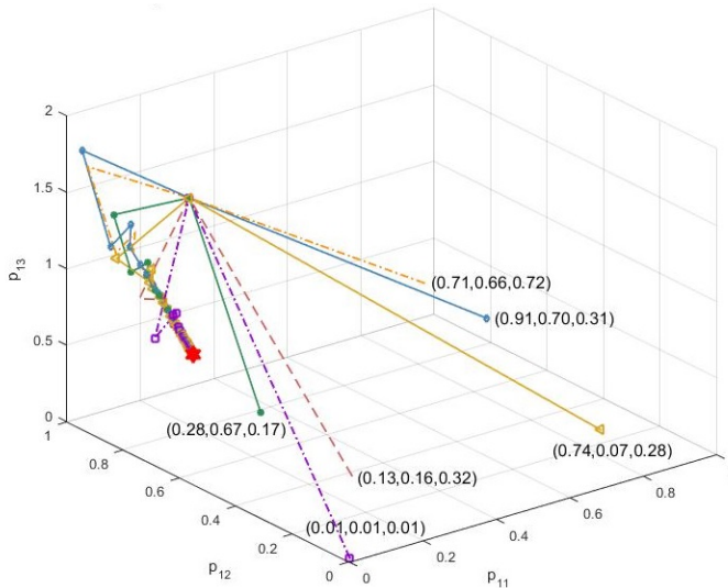
Fig. 4: Convergence of power allocation of player 1 for different starting strategies when K = 4 and M = 3 , first simulation (different linestyles correspond to different initial strategies for player 1).
