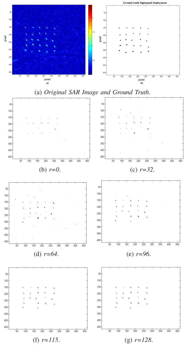
Figure 2: Original SAR image, Empirical Ground Truth and detection maps for multi-model CFAR detector, for the Sigismund deployment (Forest 2), with various censoring depths, P_{FA} = 10^{-4} and the cell size to 16 \times 16 .
